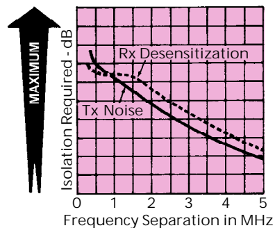
Figure 4-9: Isolation
